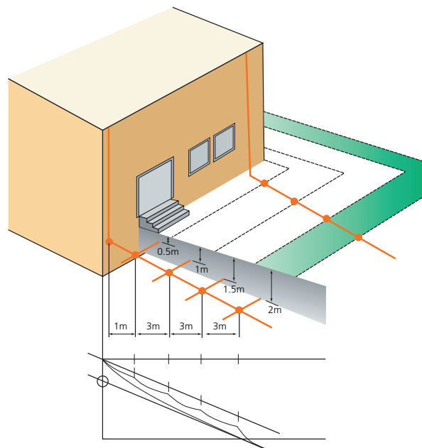
Figure 73. Ring electrodes to reduce step potential.
