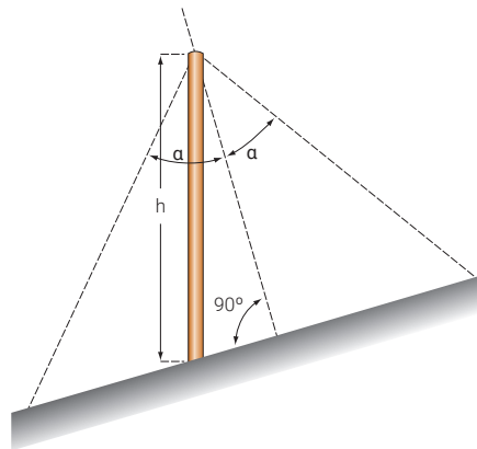
Figure 36. Protection angle method applied to inclined surface.
