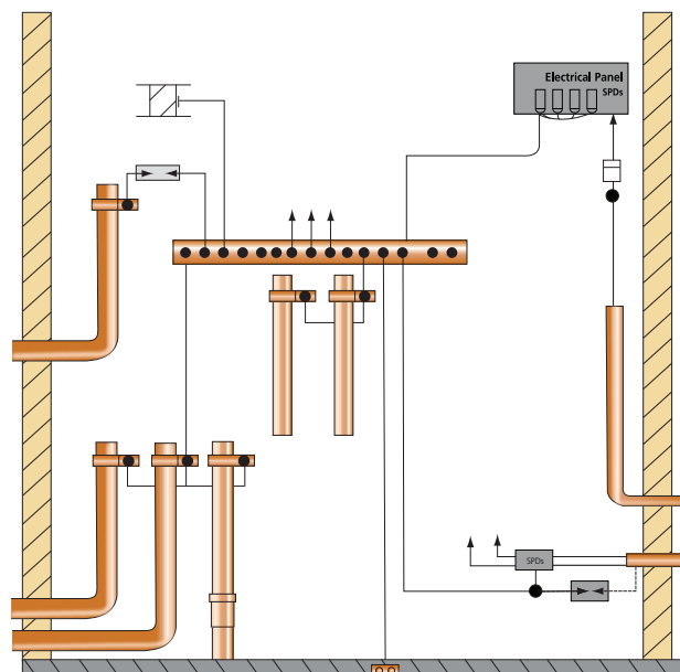
Figure 59. Bonding of services.
