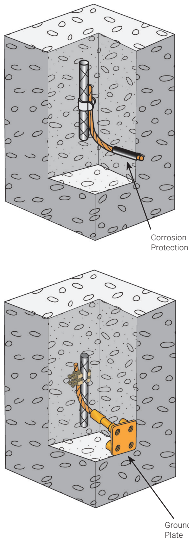
Figure 24. Ground plates are convenient and eliminate the need for corrosion protection.
