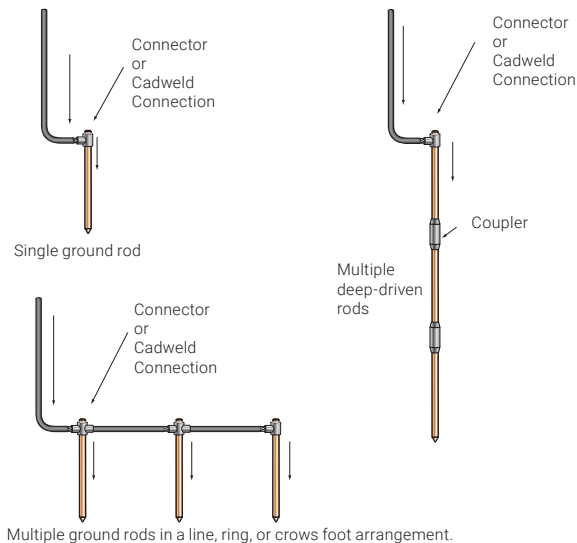
Figure 69. Example vertical electrode arrangements.
