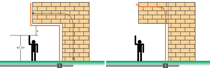
Figure 56. Overhangs.
