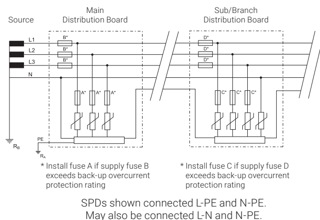
Figure 100. TN-C-S system identification.
